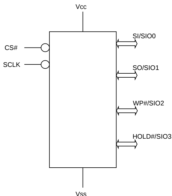
Figure 1.1 Logic Diagram
