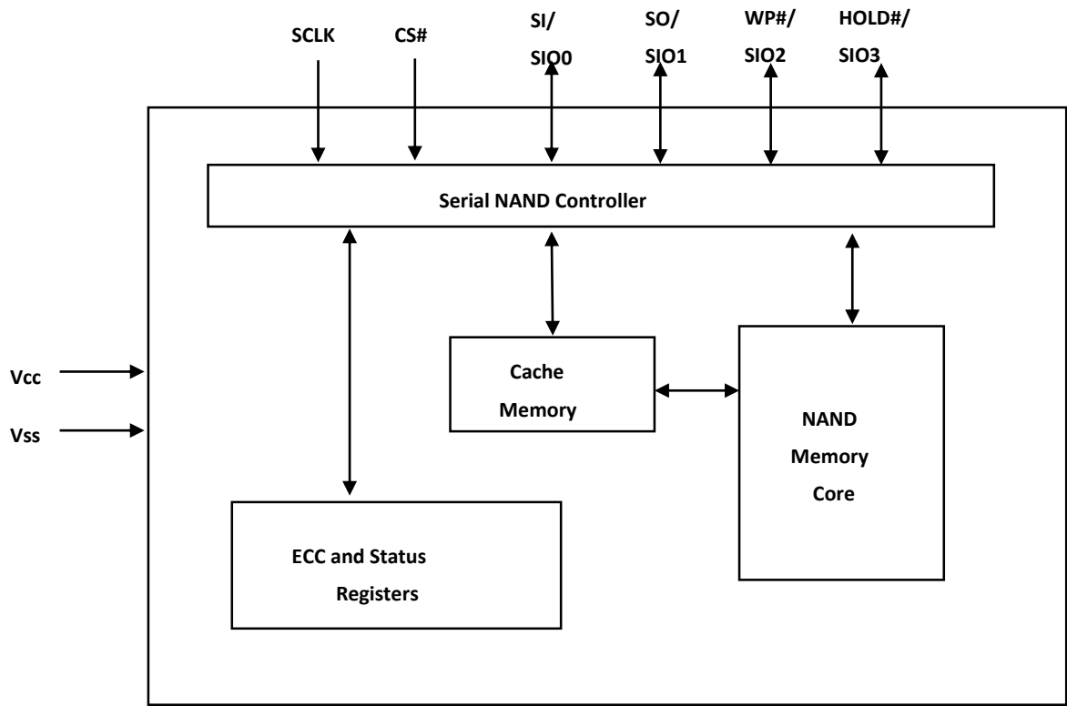
Figure 1.2 Block Description
