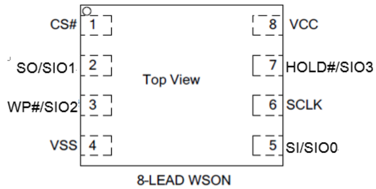
Figure 6.1 Pin Configuration
