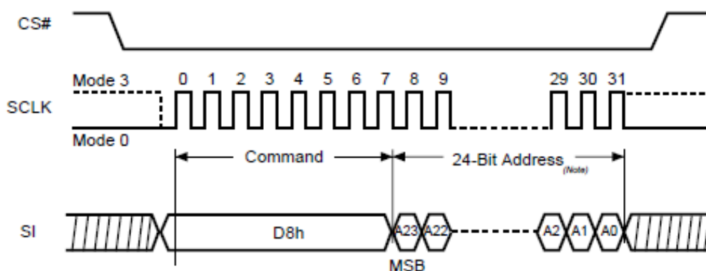
Figure 3.25 Block Erase
