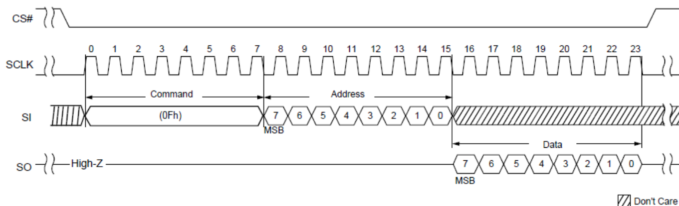
Figure 3.3 Get Features(0Fh)
