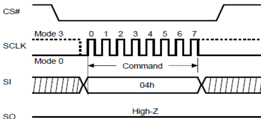
Figure 3.2 Write Disable
